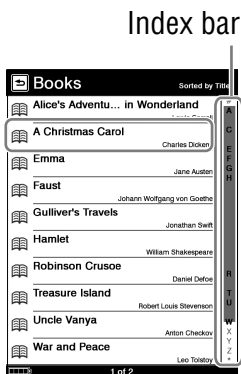
“Books” list
